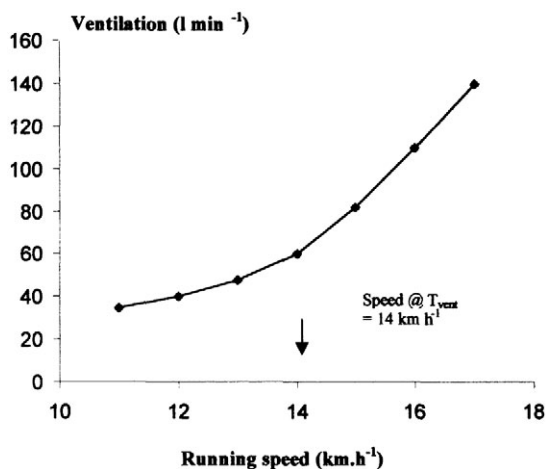
Figure 10.4 Determination of exercise intensity at ventilatory threshold ( T_{\text{vent}} ) from an incremental treadmill test.
