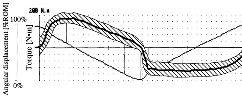
Figure 1.8 95% confidence limits constructed around a single torque-angular position curve derived from maximal voluntary muscle actions of the knee extensors and flexors at 1.05 \text{ rad s}^{-1} . The x axis denotes the time over which the muscle actions take place (approximately 3 seconds).
