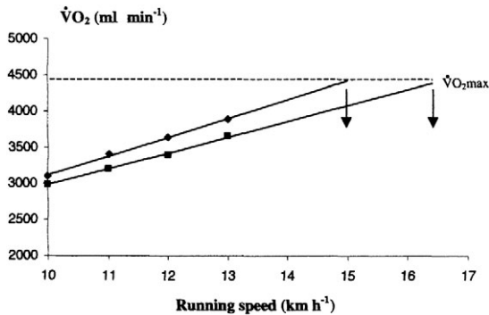
Figure 10.9 Determination of the running velocity at maximal oxygen uptake ( V\text{-}\dot{V}O_2^{\max} ). This involves regressing \dot{V}O_2 on exercise intensity for submaximal exercise and extrapolating this relationship to \dot{V}O_2^{\max} . The V\text{-}\dot{V}O_2^{\max} can differ in two individuals with the same \dot{V}O_2^{\max} (in \text{ml kg}^{-1} \text{min}^{-1} ) if exercise economy differs in the two individuals.
